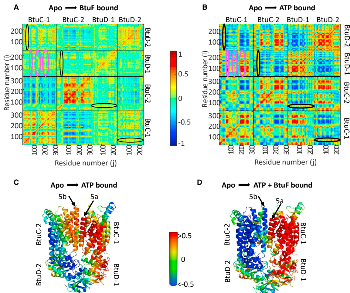
Figure 2. Binding of ATP to BtuCD Leads to Stronger Correlated Movements than Binding of BtuF
